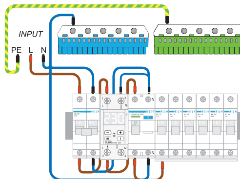
Scheme 4. Wiring diagram without a neutral bypass in ZUBR D2
