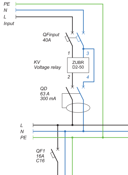
Scheme 3. Electrical diagram without a neutral bypass in ZUBR D2
