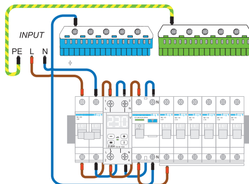
Scheme 2. Wiring diagram with a neutral bypass in ZUBR D2
