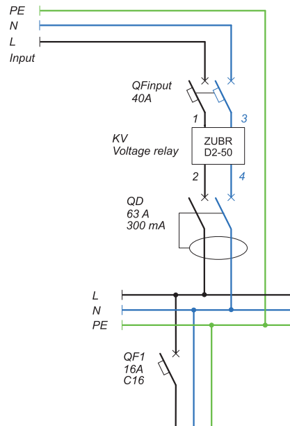
Scheme 1. Electrical diagram with a neutral bypass in ZUBR D2
